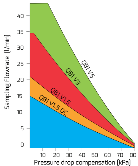
Pump characteristics
